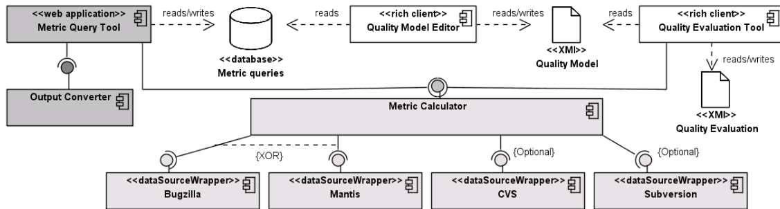
Fig. 1. Architectural Overview of the QMetric Tool Suite
